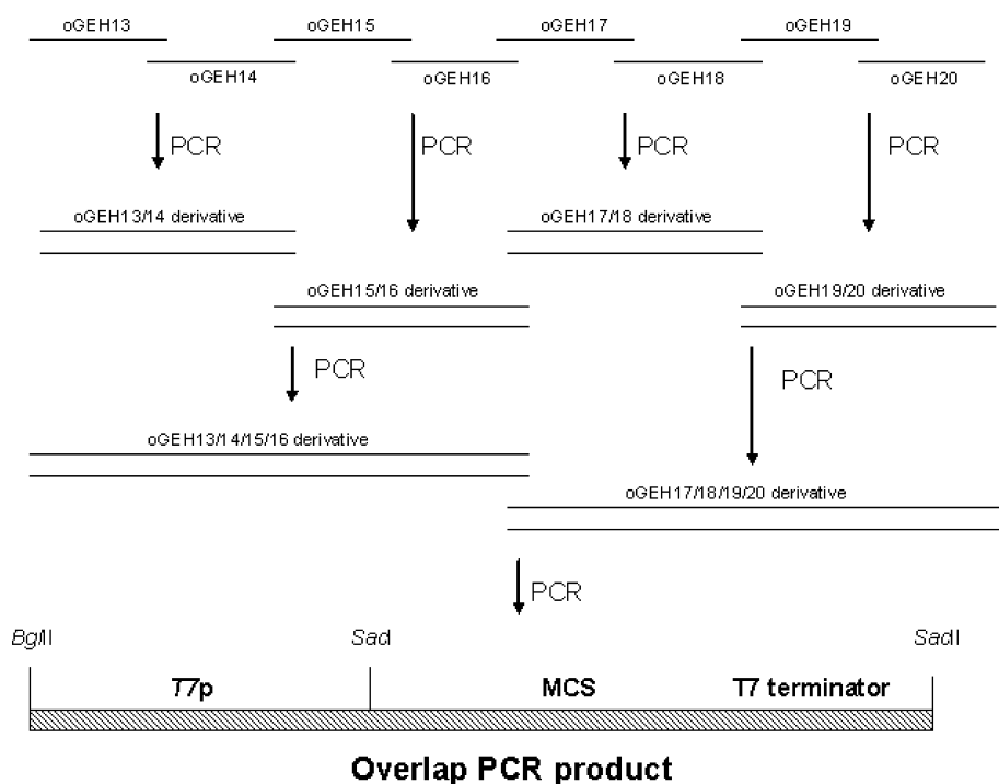
Fig. 1. Construction of overlap PCR product containing T7 promoter ( T7p ), multiple cloning site (MCS), and T7 transcriptional terminator (T7 terminator) identical to sequence in Novagen pET-3a cloning vector). Multiple PCR steps were required for complete assembly (see Materials and methods for details).
