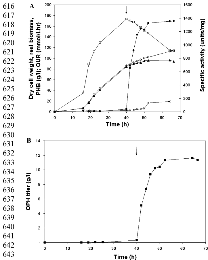
Fig. 4. Typical high cell density fermentation profile for strain GH29-8 (see Tables 1 and 3). (A) Dry cell weight (open circles), real biomass (closed triangles), PHB (crosses), O 2 uptake rate (OUR) (open squares), and OPH activity (closed circles). (B) OPH titer (closed squares). The arrow in both panels indicates the time of induction.
